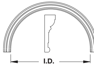
No. 150-240 Arch Height: 3 1/2" Projection: 1"
