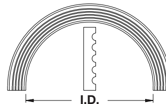
No. 150-260 Arch Height: 7 1/4" Projection: 1"
