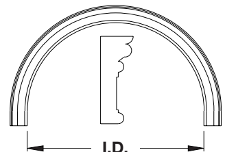
No. 150-210 Arch
