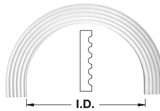
No. 150-270 Arch Height: 5 1/4" Projection: 1"
