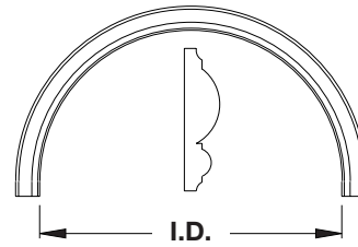
No. 150-230 Arch Height: 3" Projection: 7/8"
