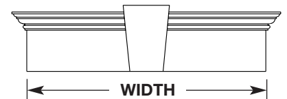
No. 750-155 Window Head Height: 9" Projection: 3"
